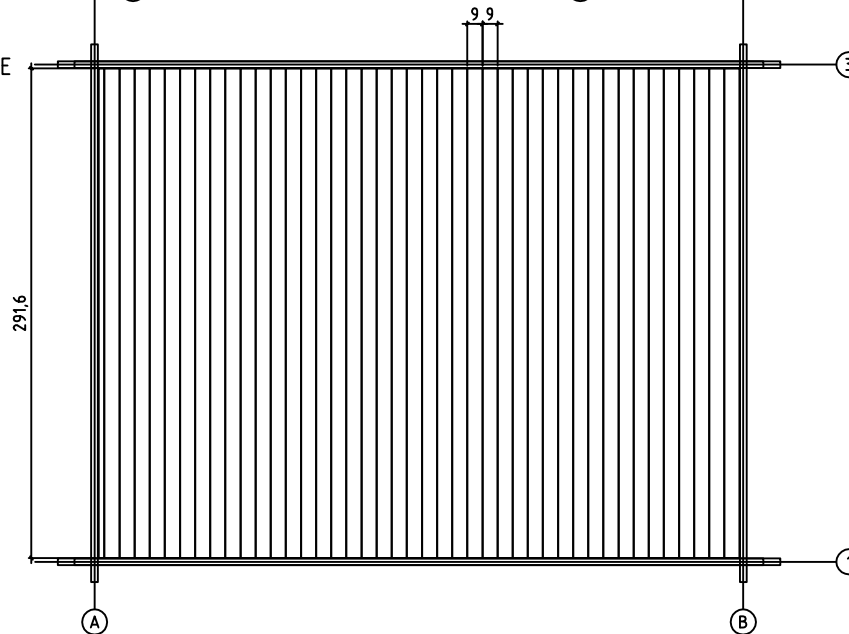
FLOOR BOARDS - - FUSSBODENBRETTER - - PLAN POSE PLANCHER
