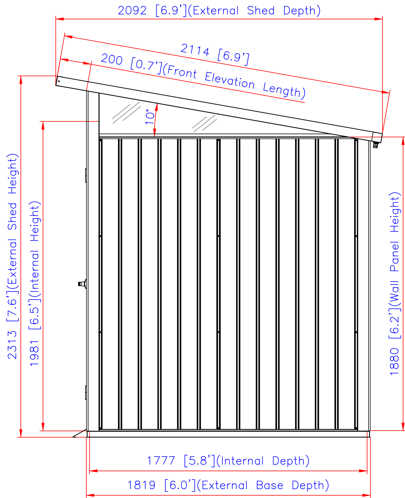
Side View
